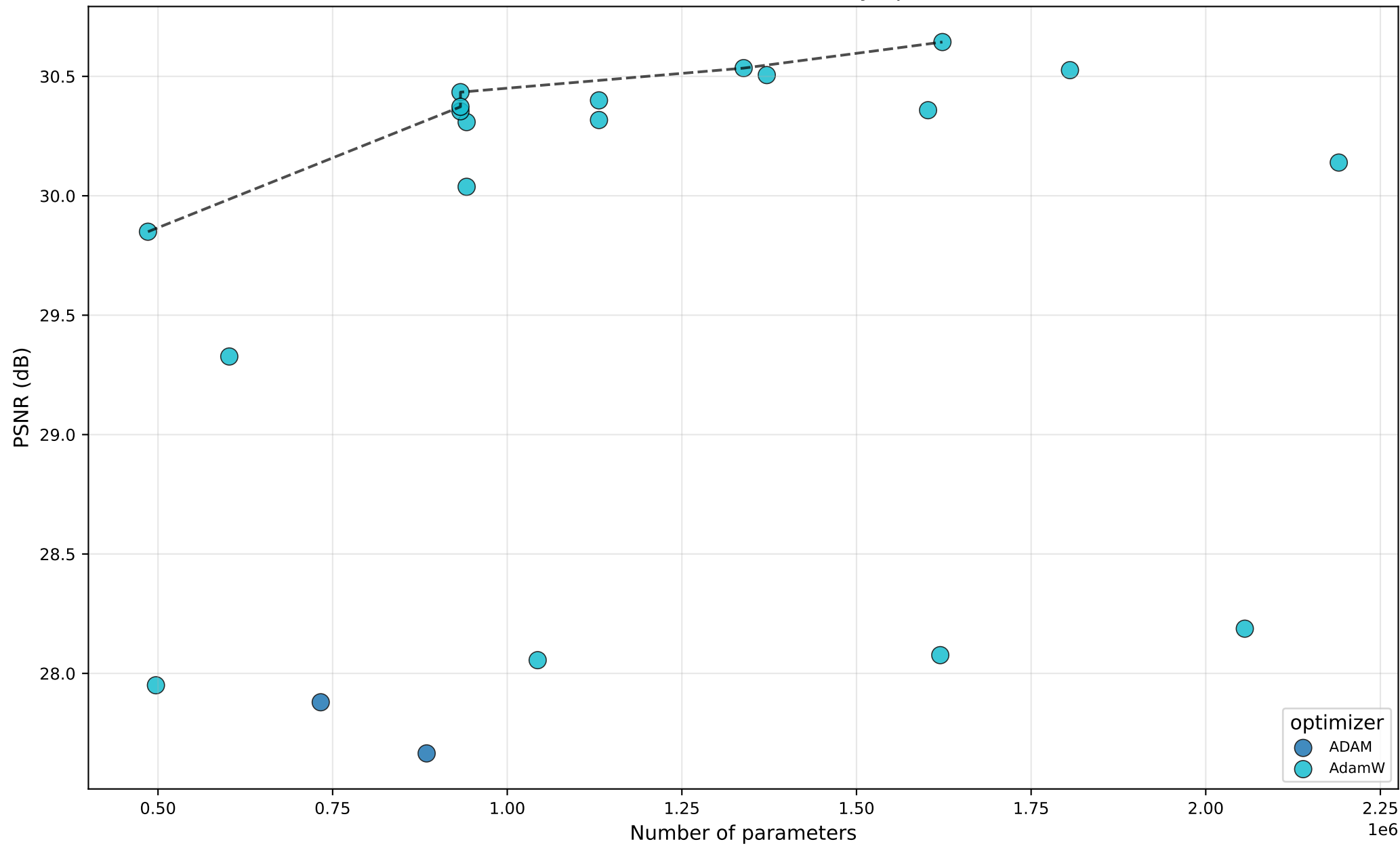
PSNR vs #Params — ELAN — by optimizer
